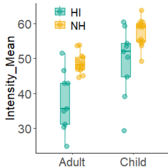
Mean intensity
