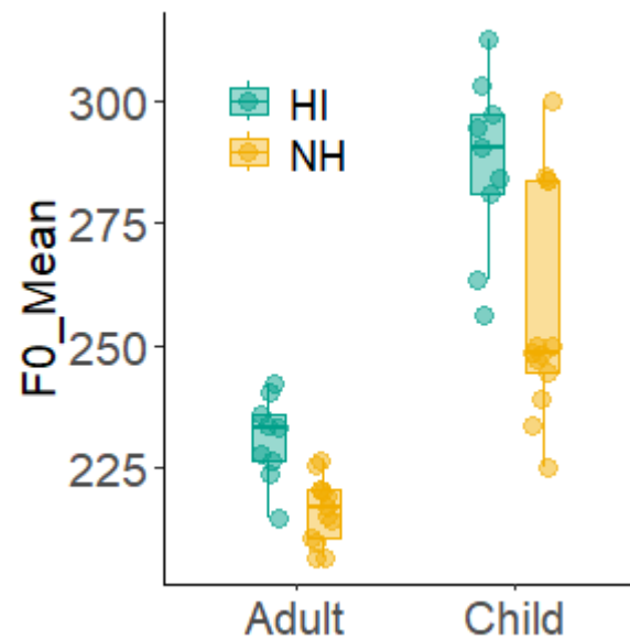
Mean F0
